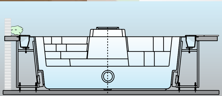
Self-supporting pool with overflow channel steel supports.
