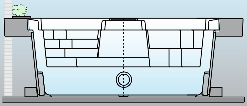
Oversized pools: Prefabricated pool with overflow channel and steel supports fixed to the pool.
